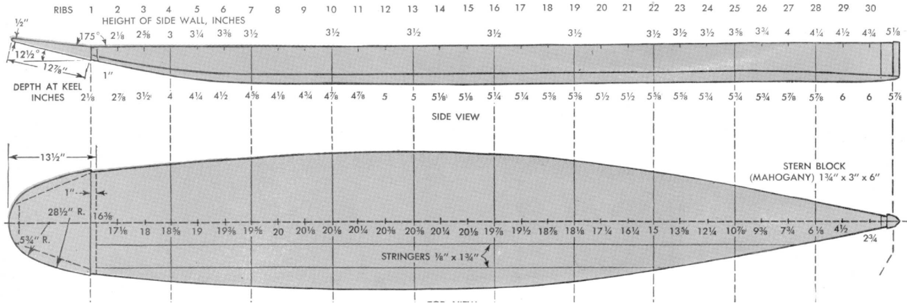
Sample of the closely spaced ribs and stringers, referred to as "Egg Crate" construction.
