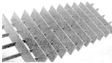
Sample of the closely spaced ribs and stringers, referred to as "Egg Crate" construction.
